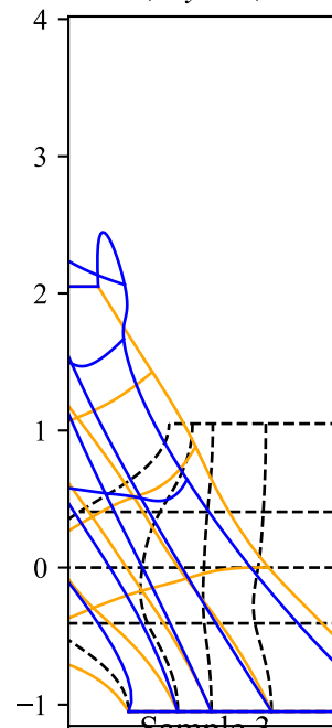
Sample 2 \Delta x = -2, \Delta y = 1, \nu = 0.18
